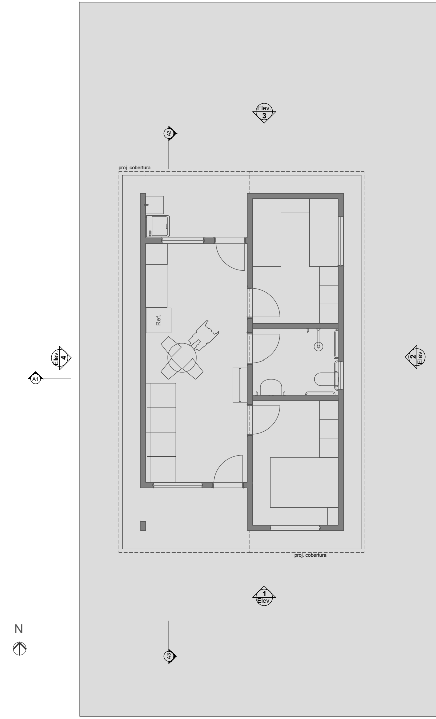
LAYOUT 1:100
